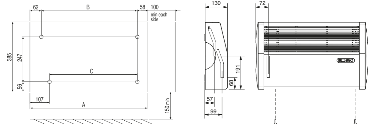
Case fixing screw positions and water connections
