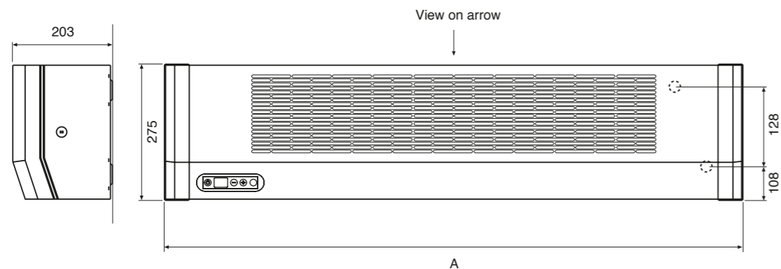
Case fixing screw positions and water connections
