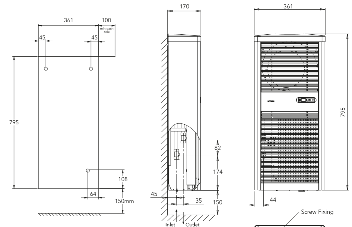
Case fixing screw positions and water connections
