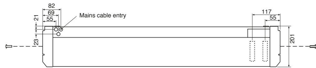
Case fixing screw positions and water connections
